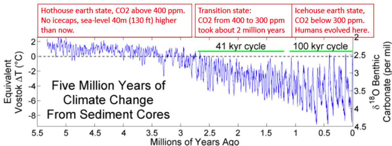
Figure 1. Five million years of climate change: It took 2 million years to transition from hothouse back to the icehouse/interglacial state (between about 3.5 to about 1.5 million years ago.)
